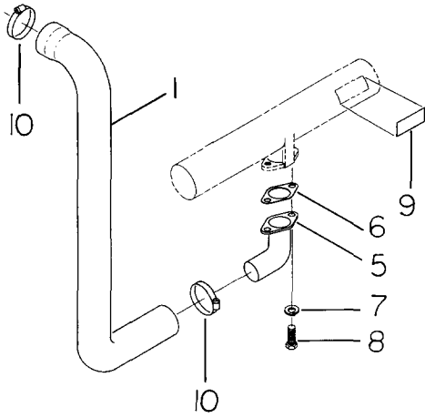
10221005 - TMD Top Mount
